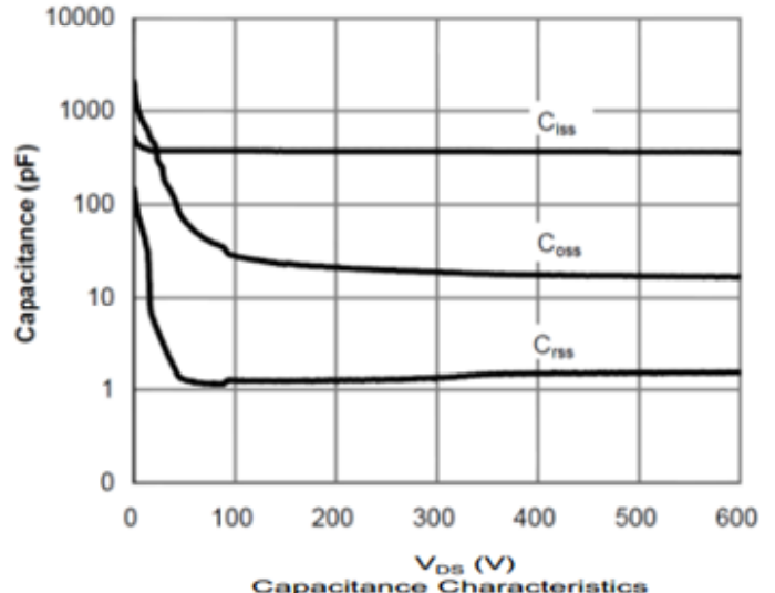
Capacitance
